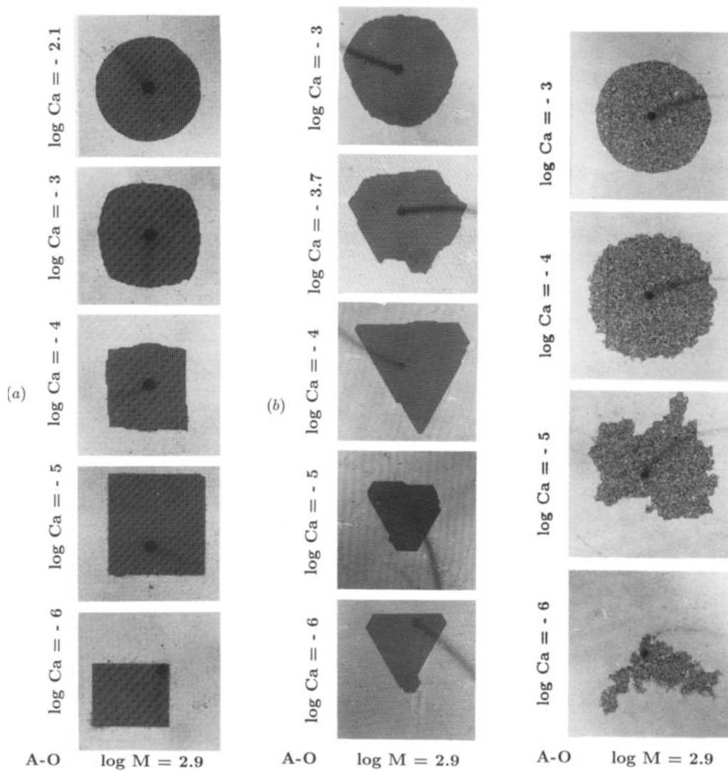
Figure 5 from R Lenormand 1990 J. Phys.: Condens. Matter 2 SA79
